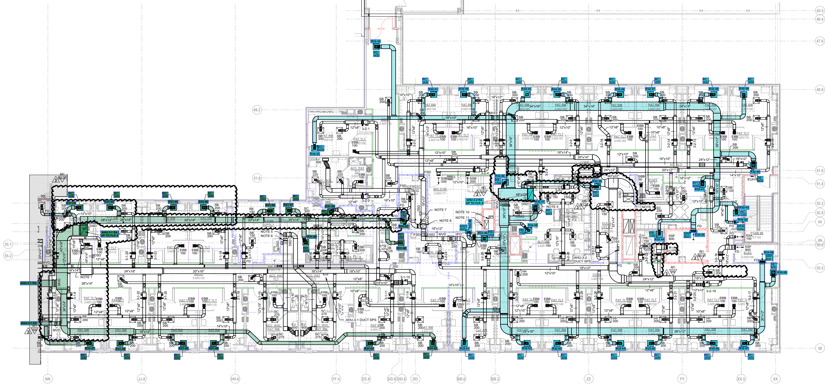
3RD FLOOR HVAC FLOOR PLAN - PART B
