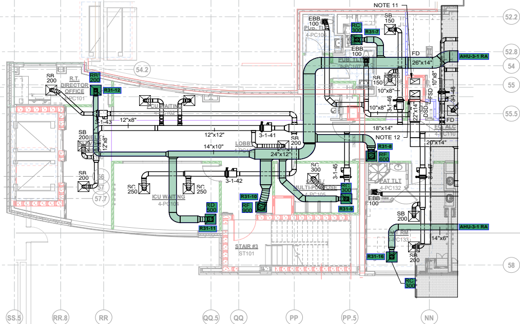
4TH FLOOR HVAC FLOOR PLAN - PART A SCALE: 1/8" = 1'-0"
