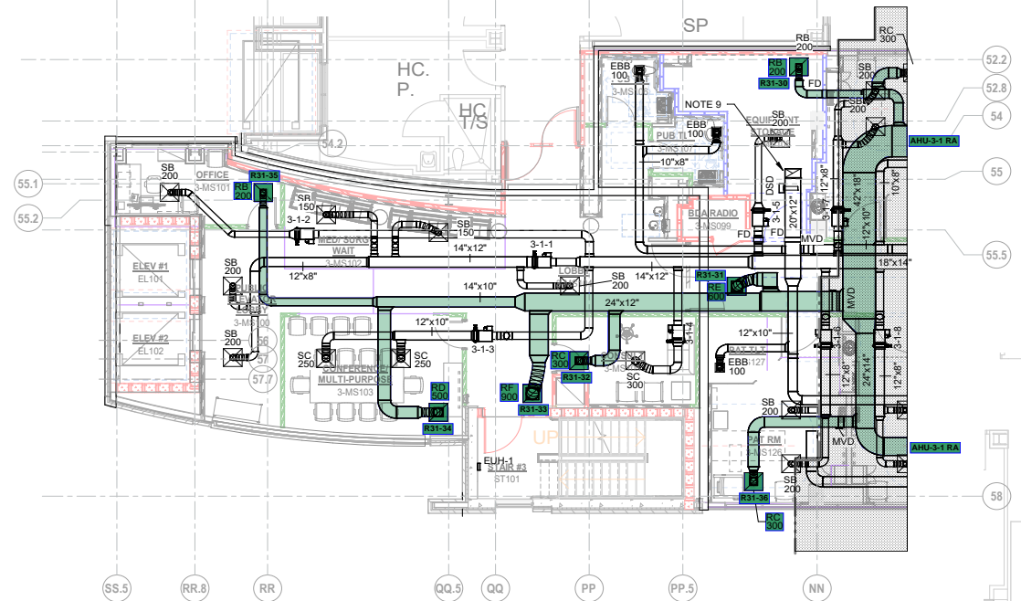
3RD FLOOR HVAC FLOOR PLAN - PART A SCALE: 1/8" = 1'-0"
