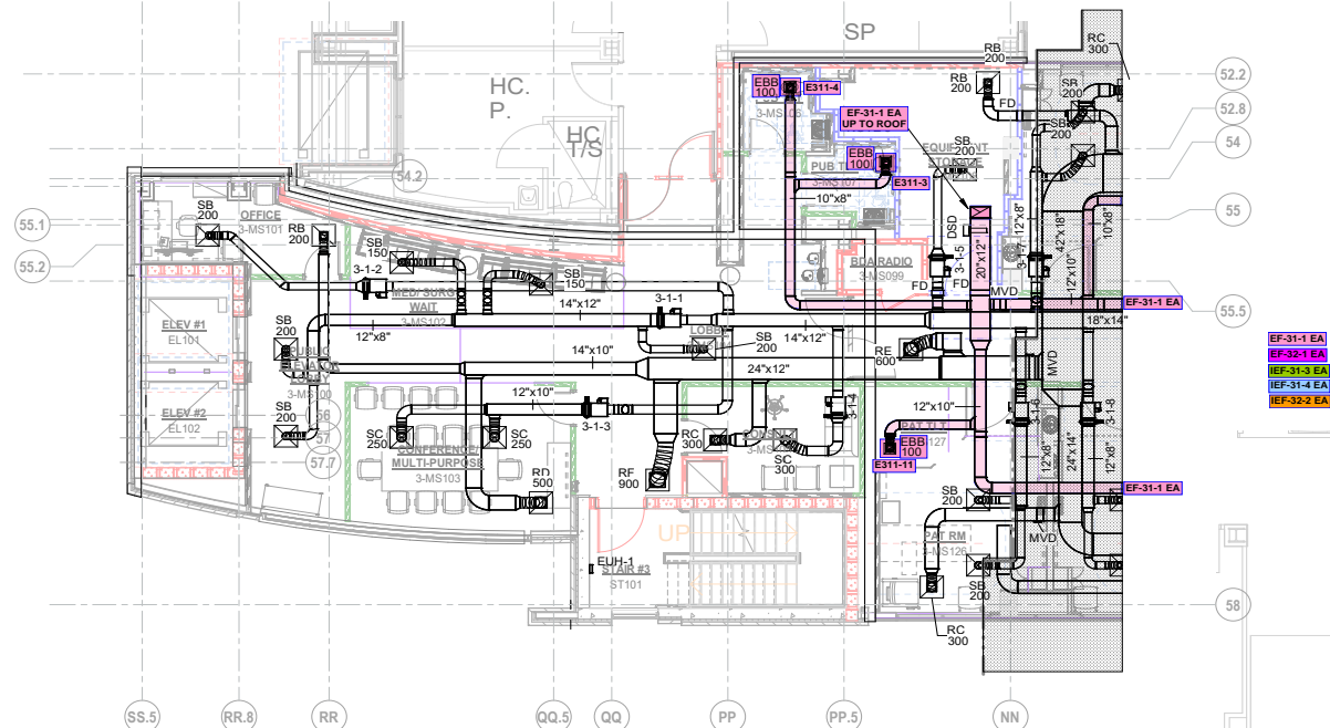
3RD FLOOR HVAC FLOOR PLAN - PART A SCALE: 1/8" = 1'-0"
