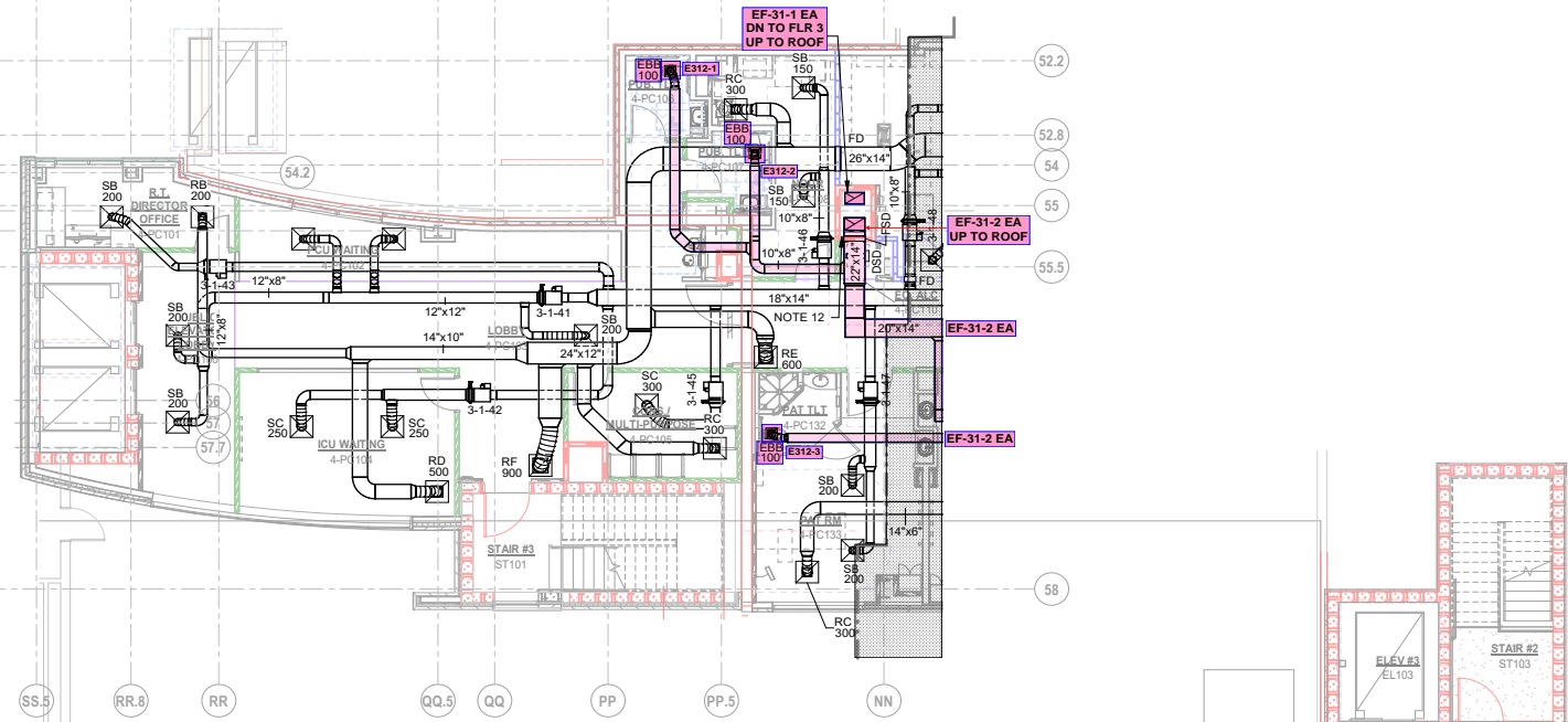
4TH FLOOR HVAC FLOOR PLAN - PART A SCALE: 1/8" = 1'-0"
