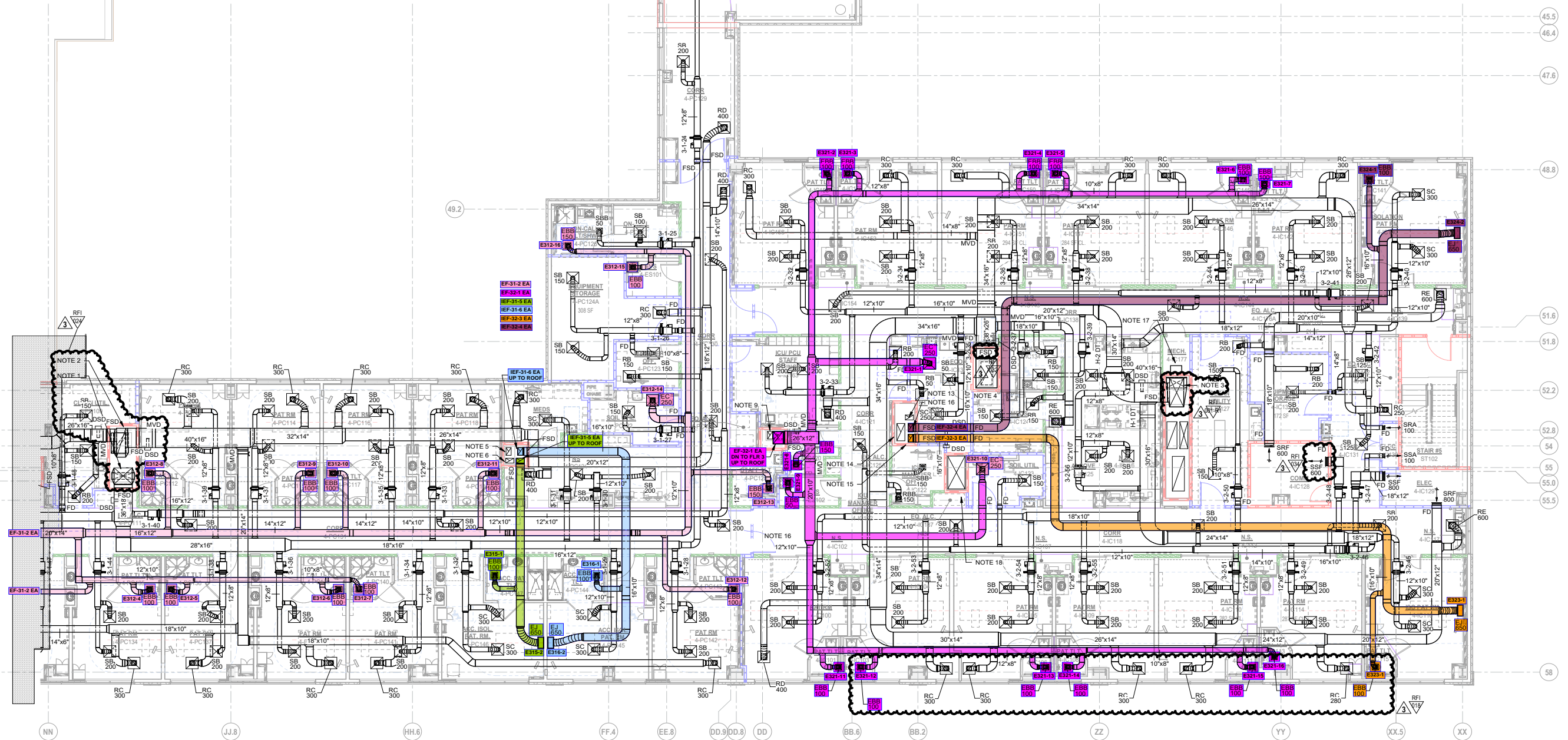
4TH FLOOR HVAC FLOOR PLAN - PART B
